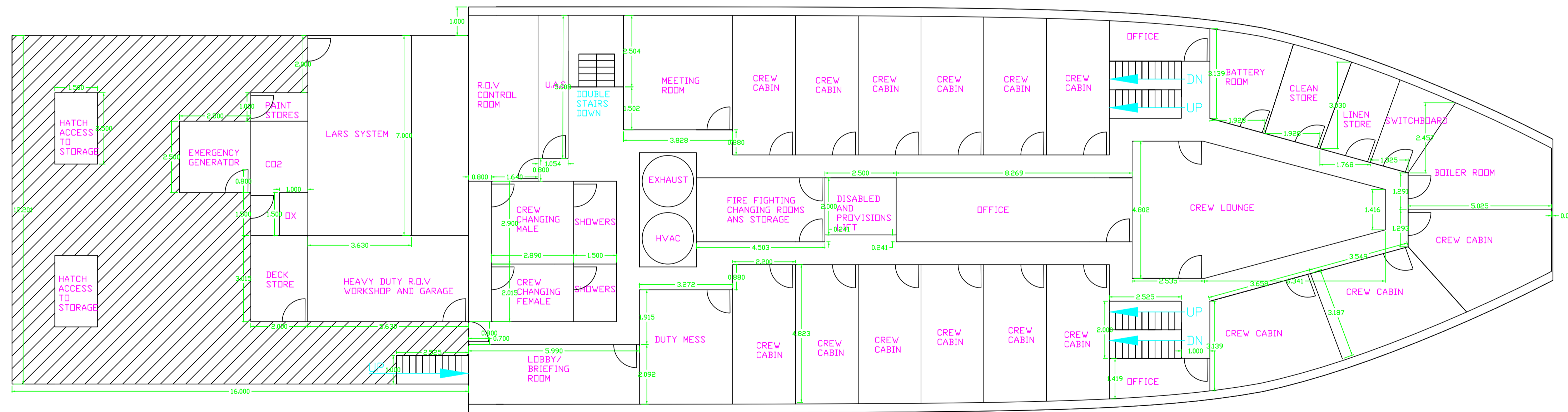
1 DECK - MAIN
